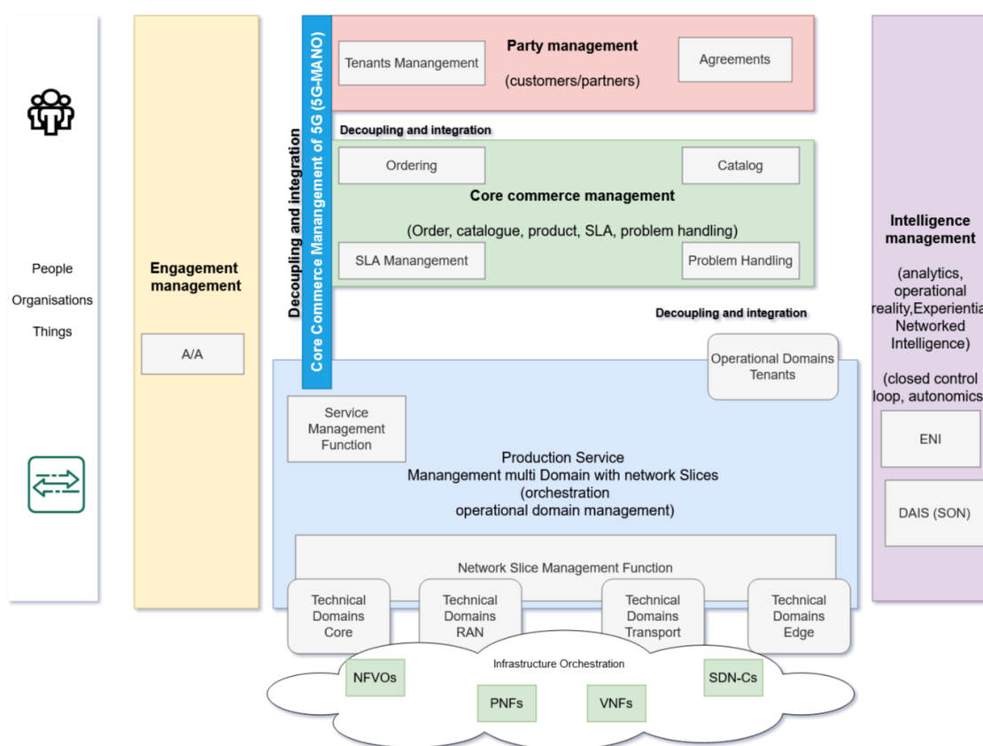
Figure C.2: 5G architecture mapped to the ODA functional blocks
