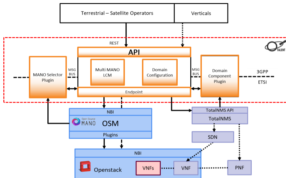
Figure C.3: TALENT architecture
