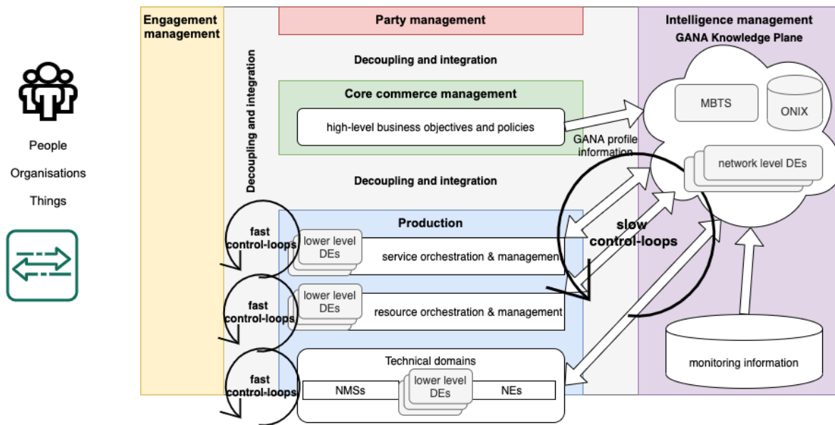
Figure B.27: ETSI GANA components mapped to the ODA functional blocks
